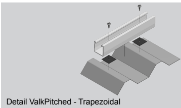
Detail ValkPitched - Trapezoidal
