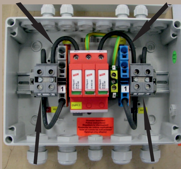
+ Inverter
